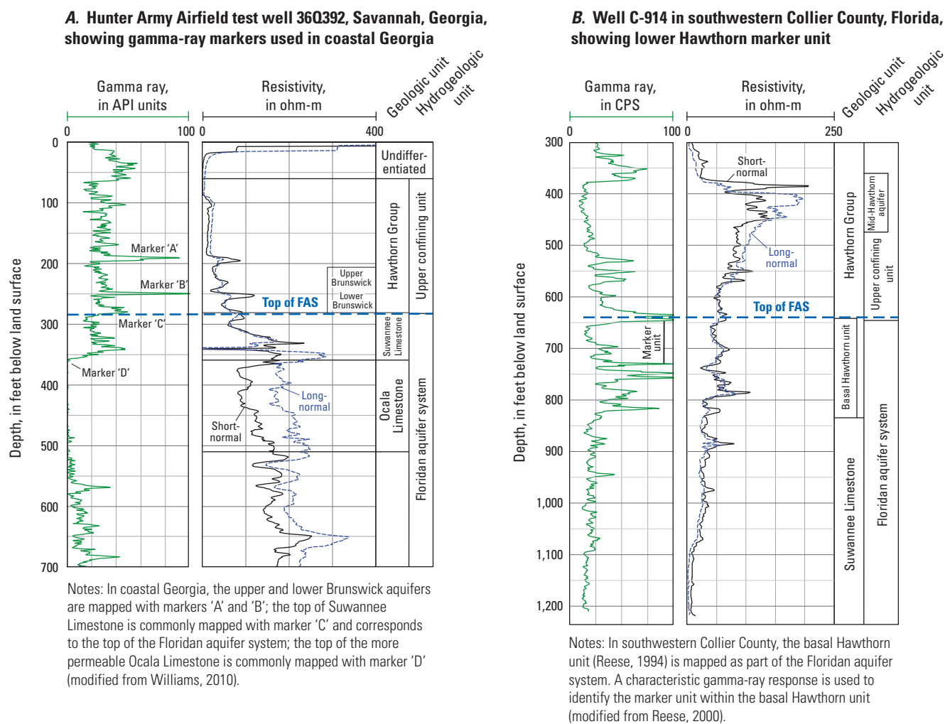
Figure 15. Geophysical marker horizons used for mapping hydrogeologic units in the Floridan aquifer system. [API, American Petroleum Institute; ohm-m, ohm-meter; CPS, counts per second; FAS, Floridan aquifer system; well locations shown on plate 1]
